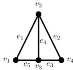
Figure 2. graph \Upsilon_2
