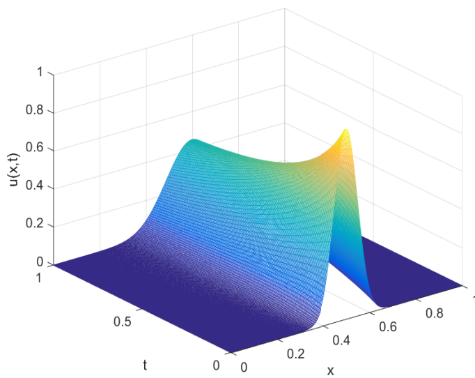
Fig. 15 The exact solution for SPDE (19) with the parameters \gamma = 0.005 , \nu = 0.1 , and \sigma = 0.03 .
