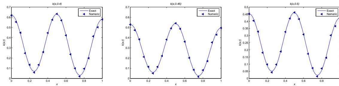
Figure 2. Comparison between the exact and numerical results for k(x, 0.4) , k(x, 0.45) , and k(x, 0.5) , in Example 1, with the given data (18)-(24) when \Delta x = 0.01 .
