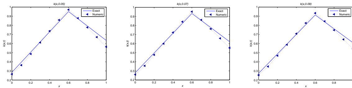
Figure 4. Comparison between the exact and numerical results for k(x, 0.05) , k(x, 0.07) , and k(x, 0.09) , in Example 2, with the given data (25)-(31) when \Delta x = 0.01 .
