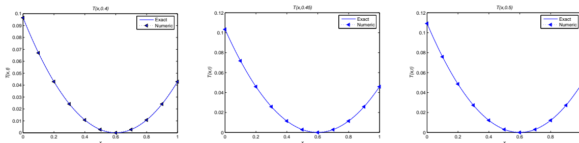
Figure 1. Comparison between the exact and numerical results for T(x,0.4) , T(x,0.45) , and T(x,0.5) , in Example 1, with the given data (18)-(24) when \Delta x = 0.01 .
