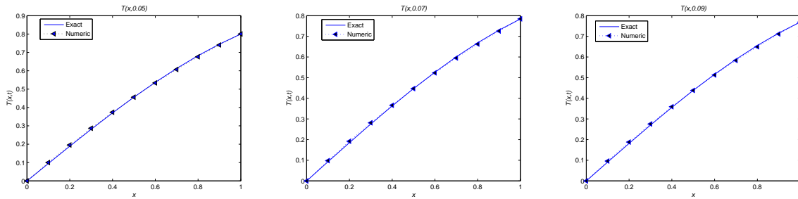
Figure 3. Comparison between the exact and numerical results for T(x, 0.05) , T(x, 0.07) , and T(x, 0.09) , in Example 2, with the given data (25)-(31) when \Delta x = 0.01 .
