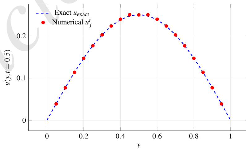
Figure 5. Comparison of the exact and numerical solutions along the temporal slice t = 0.5 with N = 64 , n = 16 , and M = 8 .
