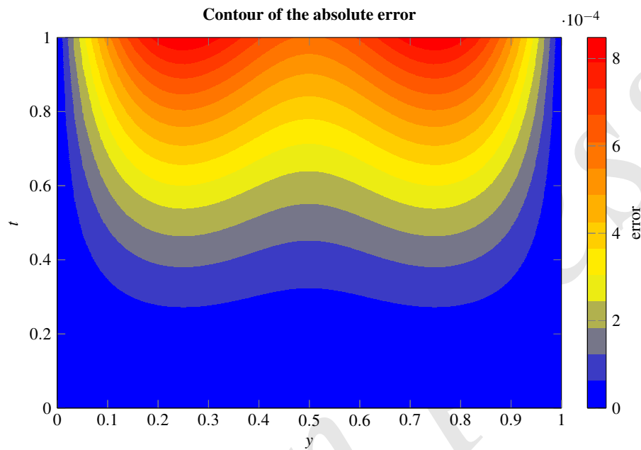
Figure 4. Filled contour plot of the absolute error |u_{\text{exact}}(y, t) - u_j^r| in the (y, t) plane, using the same parameters as in Figure 3.
