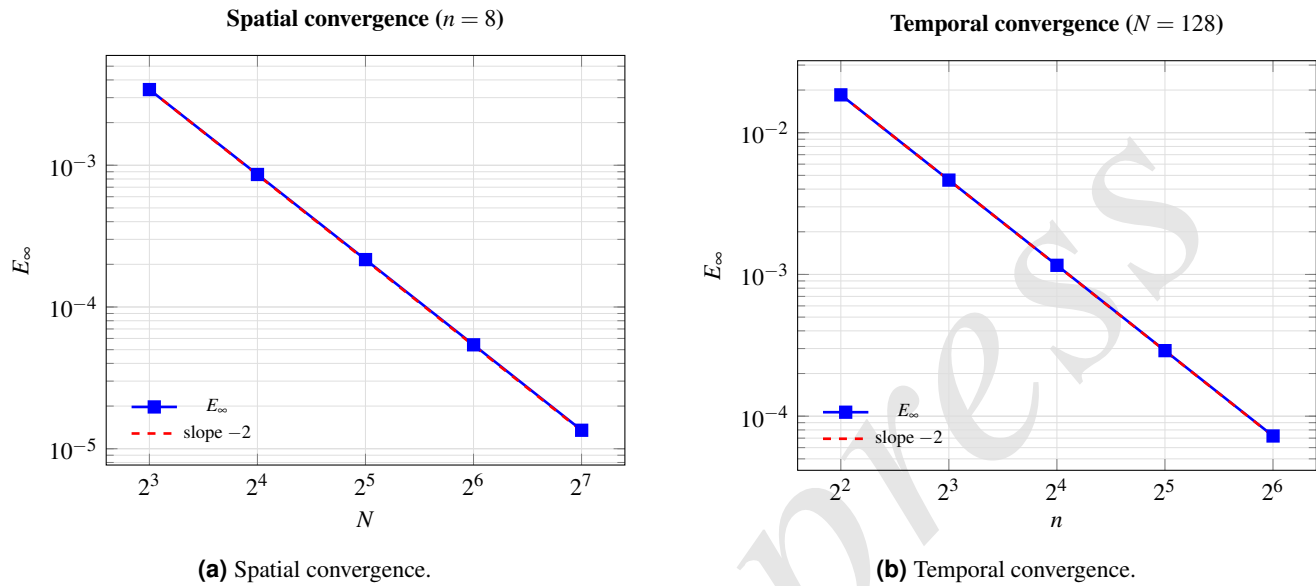
Figure 6. Log-log convergence plots corresponding to the data of Table 1 and Table 2. The dashed reference lines of slope -2 confirm the second-order accuracy in both space and time.
