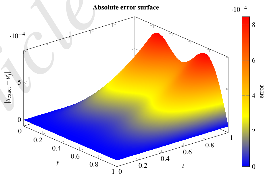
Figure 3. Absolute error surface |u_{\text{exact}}(y, t) - u_j^r| for the same parameters as in Figure 1.
