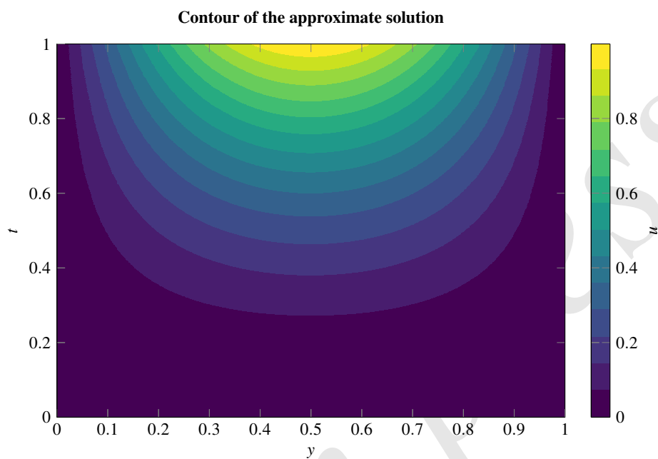
Figure 2. Filled contour plot of the approximate solution u_j^r in the (y, t) plane, using the same parameters as in Figure 1.
