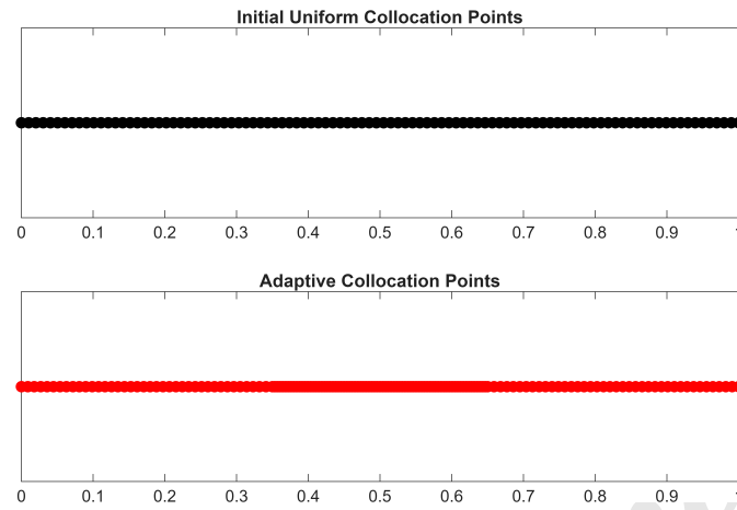
Figure 4. Distribution of collocation points before and after adaptive refinement. Additional points are concentrated in regions identified by the kernel-aware difficulty indicator as numerically demanding.
