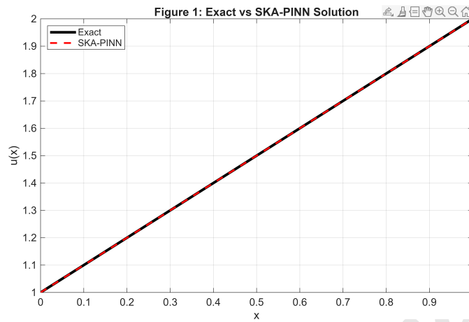
Figure 1. Comparison of the exact analytical solution and the SKA-PINN prediction for the weakly singular Fredholm integral equation. The two curves are almost indistinguishable over the computational domain, indicating close agreement between the numerical and analytical solutions.
