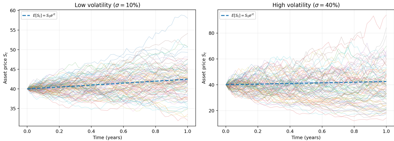
Figure 4. Simulated Geometric Brownian (motion Asset Paths—under Low- and High-Volatility Market Conditions)
