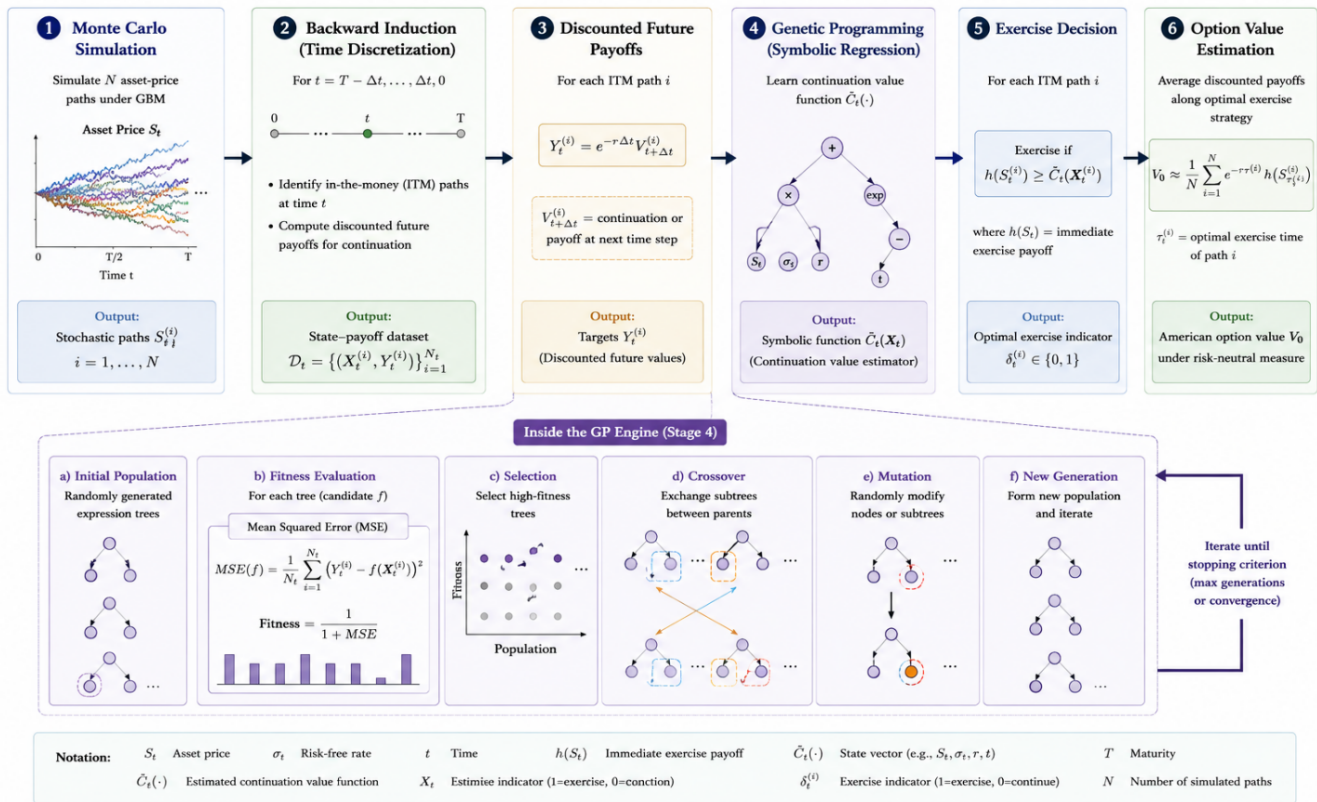
Figure 3. Computational Workflow of the Proposed Monte Carlo–Genetic Programming (MCGP) Framework
