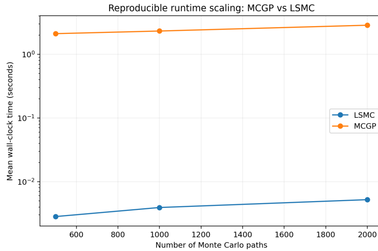
Figure 9. Reproducible Runtime Scaling of MCGP and LSMC
