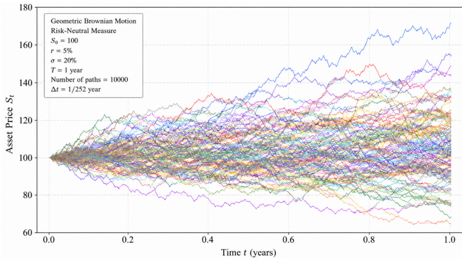
Figure 1. Simulated Geometric Brownian motion Asset Paths under Risk-Neutral Measure
