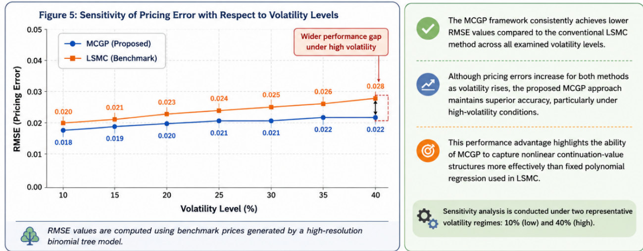
Figure 5. Sensitivity of Pricing Error with Respect to Volatility Levels
