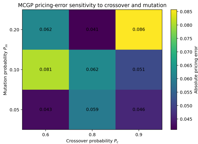
Figure 7. Pricing-Error Heatmap for Crossover and Mutation Probabilities
