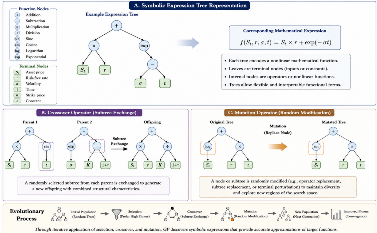
Figure 2. Symbolic Representation and Evolutionary Optimization Process in Genetic Programming
