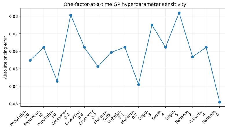
Figure 6. One-Factor-at-a-Time GP Hyperparameter Sensitivity
