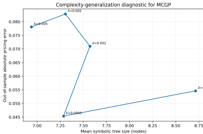
Figure 8. Complexity–Generalization Diagnostic for MCGP
