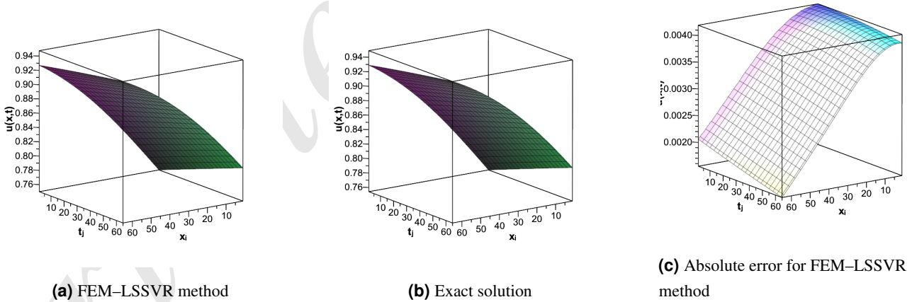
Figure 3. Numerical results for Example 2 with 64 elements: x_i \in [0, 5] , i = 0, \dots, 64 ; t_j \in [0, 1] , j = 0, \dots, 64 .
