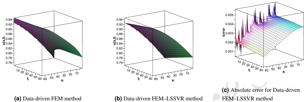
Figure 4. Comparison of numerical results for Example 2 in the noisy setting with 64 elements: x_i \in [0, 5] , i = 0, \dots, 64 ; t_j \in [0, 1] , j = 0, \dots, 64 .
