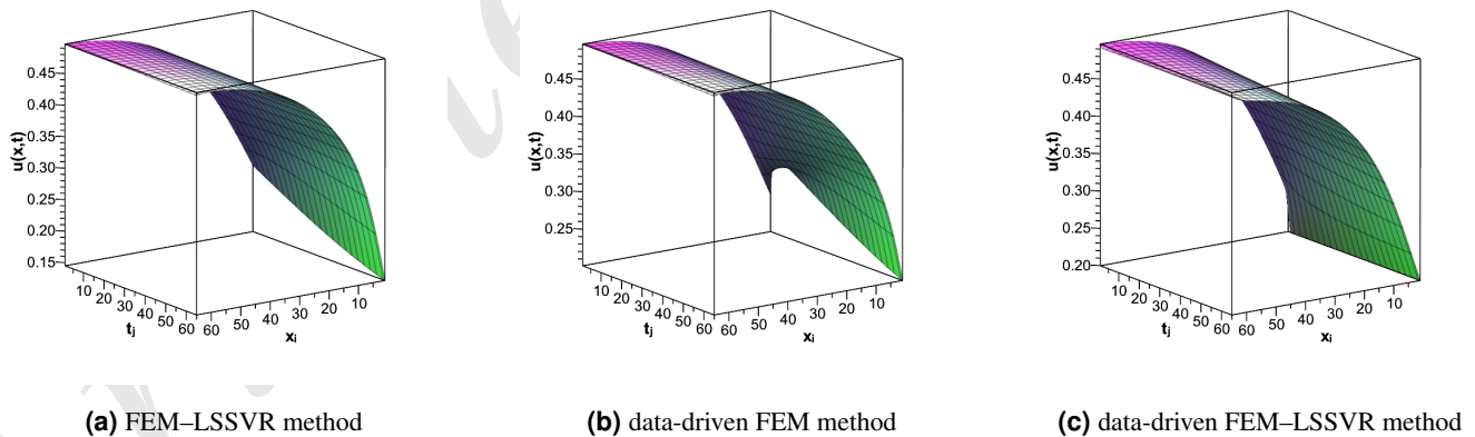
Figure 5. Comparison of numerical results for Example 3 with 64 elements: x_i \in [0, 10] , i = 0, \dots, 64 ; t_j \in [0, 1] , j = 0, \dots, 64 .
