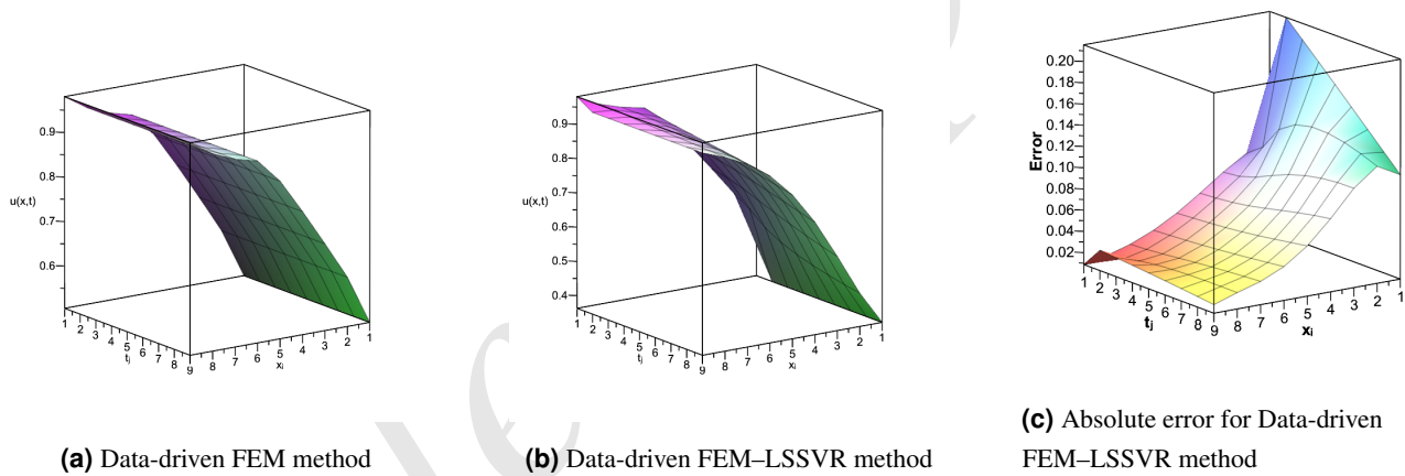
Figure 7. Comparison of numerical results for Example 4 in the noisy setting with 8 elements: x_i \in [0, 5] , i = 0, \dots, 8 ; t_j \in [0, 1] , j = 0, \dots, 8 .
