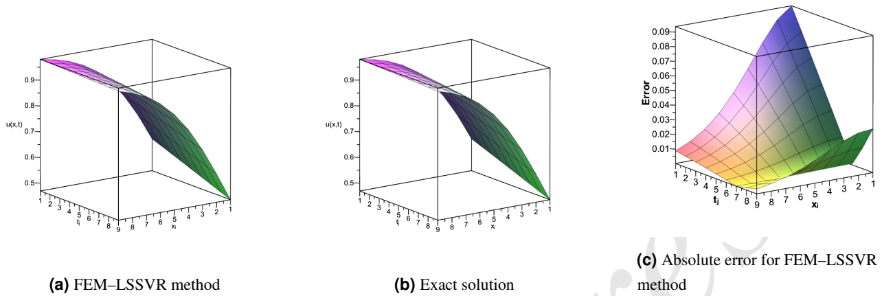
Figure 6. Numerical results for Example 4 with 8 elements: x_i \in [0, 5] , i = 0, \dots, 8 ; t_j \in [0, 1] , j = 0, \dots, 8 .
