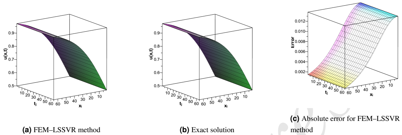
Figure 1. Numerical results for Example 1 with 64 elements: x_i \in [0, 5] , i = 0, \dots, 64 ; t_j \in [0, 1] , j = 0, \dots, 64 .
