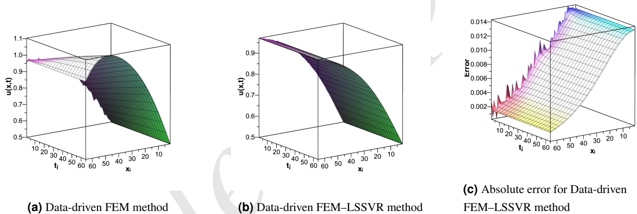
Figure 2. Comparison of numerical results for Example 1 in the noisy setting with 64 elements:
