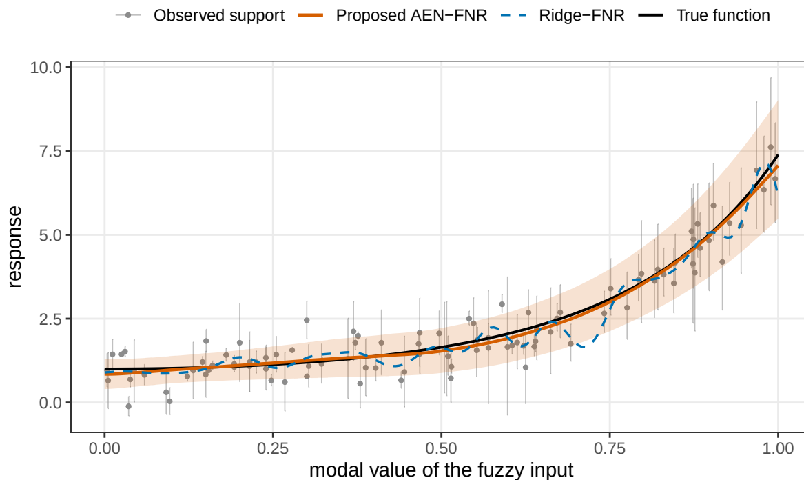
Figure 2. Example 1, one replication. Grey segments show the supports of the observed fuzzy responses at their modal inputs, the black curve is the true function, the orange band is the fitted support of the proposed AEN-FNR, the orange curve its fitted modal value, and the dashed blue curve the fitted modal value of the ridge regularized baseline. The proposed fit tracks the sharp growth of \exp(2x^2) near the right boundary without the oscillation that uniform ridge shrinkage leaves behind.
