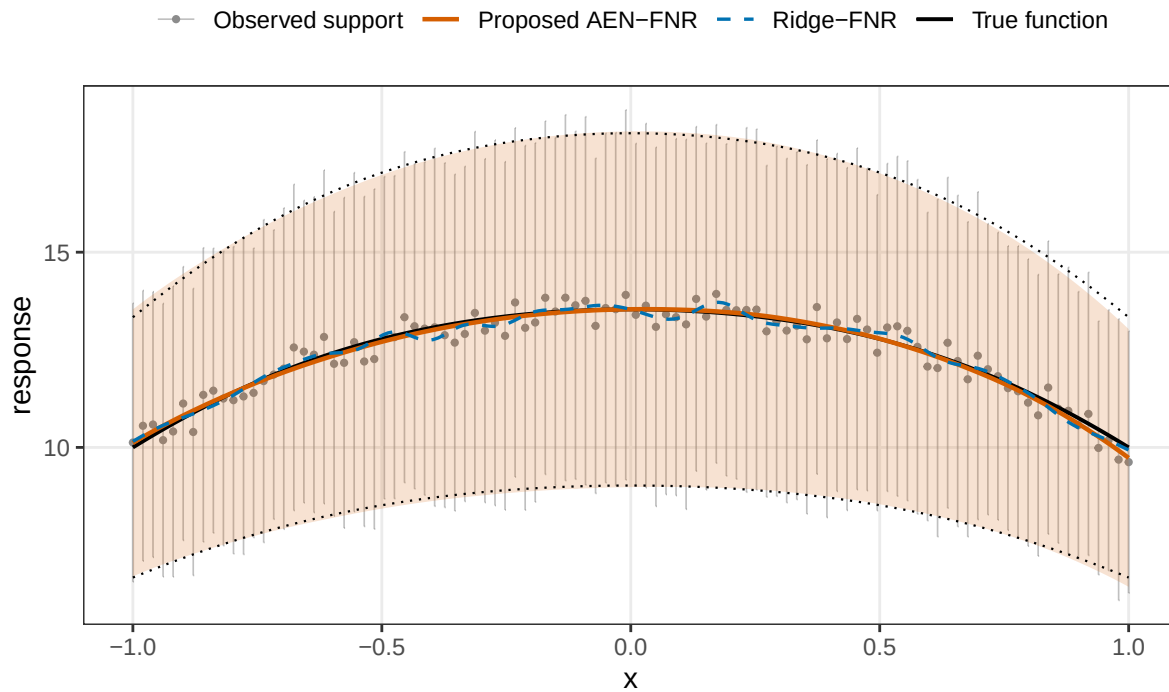
Figure 4. Example 3, one replication. Grey segments show the observed triangular responses, the black solid curve the true center g , the dotted curves the true support, the orange band the fitted support of the proposed method with its center curve, and the dashed blue curve the ridge baseline center. The fitted support respects the ordering and nestedness constraints by construction.
