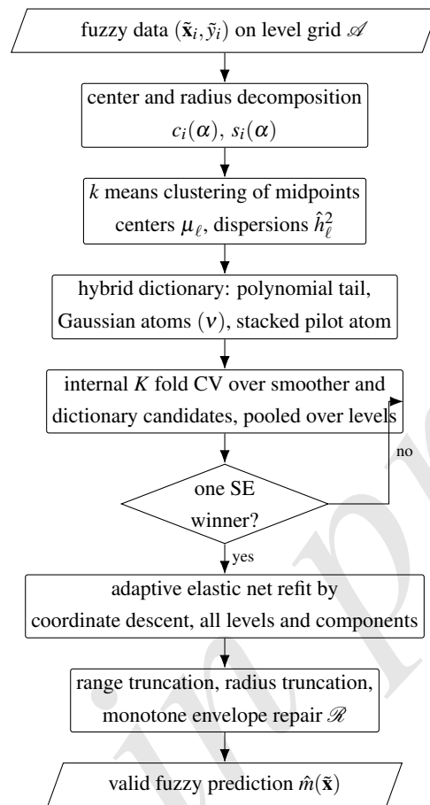
Figure 1. Flowchart of the proposed AEN-FNR procedure. The inner loop selects the dispersion rescaling and the sparsity level for each component, shared across membership levels; the outer path produces a shape-valid fuzzy prediction.
