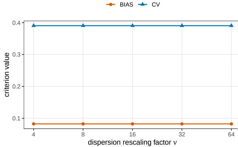
Figure 5. Example 3: cross validation error and bias of the proposed method as functions of the dispersion rescaling factor v when v is held fixed. The internal selection recovers the region of the optimum automatically.
