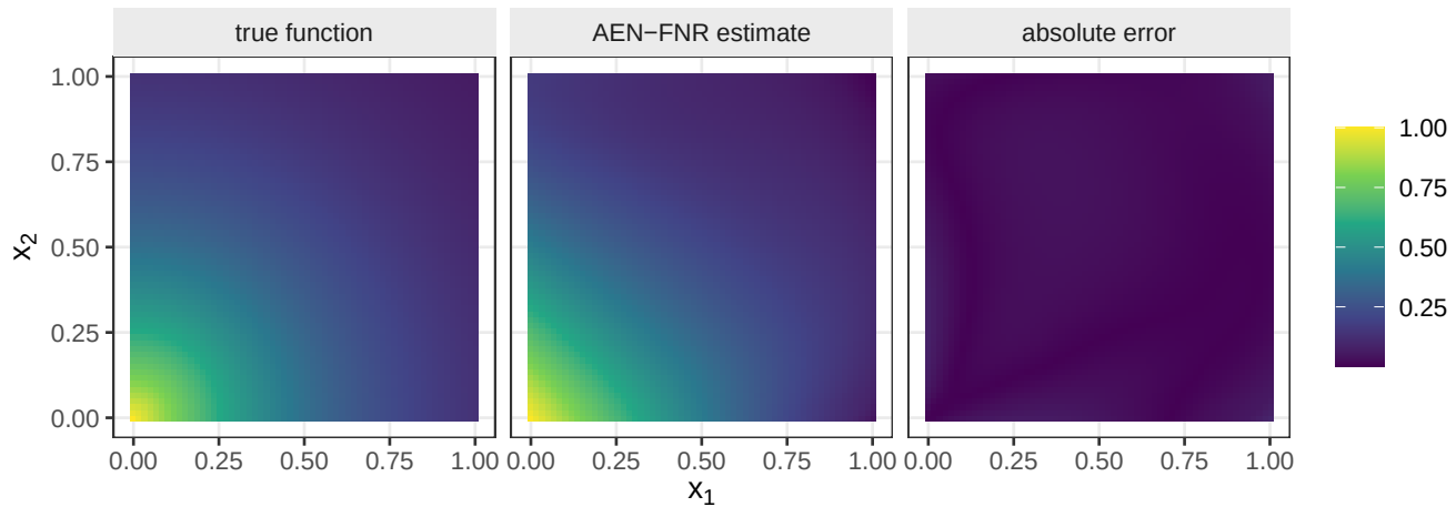
Figure 3. Example 2, one replication. Left: true surface m(x_1, x_2) = \exp(-2\sqrt{x_1^2 + x_2^2}) . Middle: modal surface estimated by the proposed method. Right: absolute error. The error concentrates in the corner of steepest curvature and stays an order of magnitude below the signal range elsewhere.
