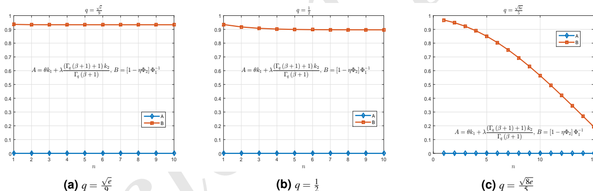
Figure 2. Graphical representation of A and B of q -FL-EPP (20) for q = \frac{\sqrt{e}}{9}, \frac{1}{2}, \frac{\sqrt{8e}}{5} .
