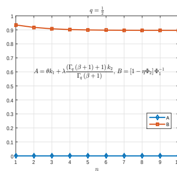
(b) q = \frac{1}{2}
