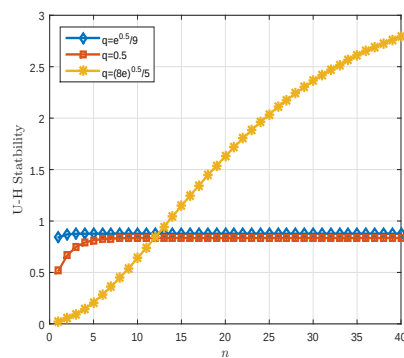
(a) UH Stability
