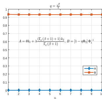
(a) q = \frac{\sqrt{e}}{9}
