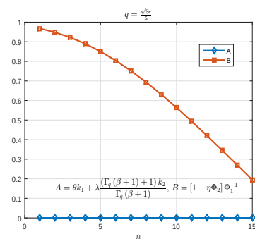
(c) q = \frac{\sqrt{8e}}{5}
